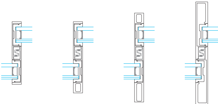
Handles frames
