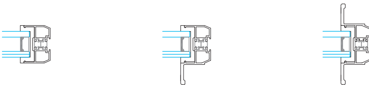
Angle frame
