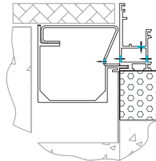
Channels
