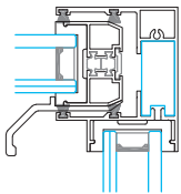
Angle frame
