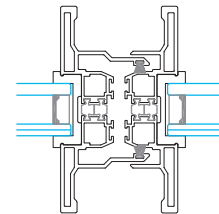
Center opening
